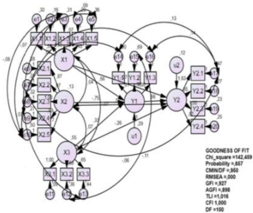
Diagram Path Full Model Structural Model Testing (Model 2 (end))
