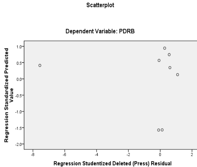
Figure 3 . Heteroscedasticity Test Results Source: Secondary Data Processed 2019
