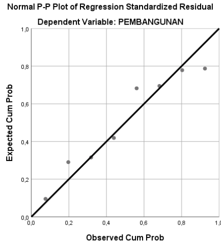
Figure 2. Normality Test Results Source: Secondary Data Processed 2019
