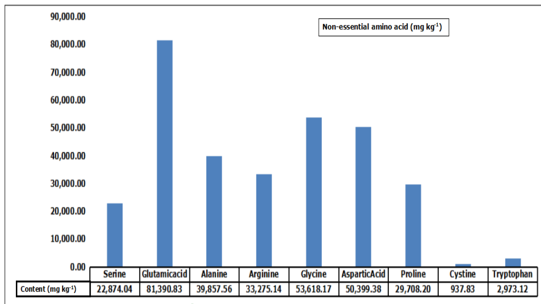
Figure 2. The profiles of non-essential amino acid in Telmatherina bonti .
