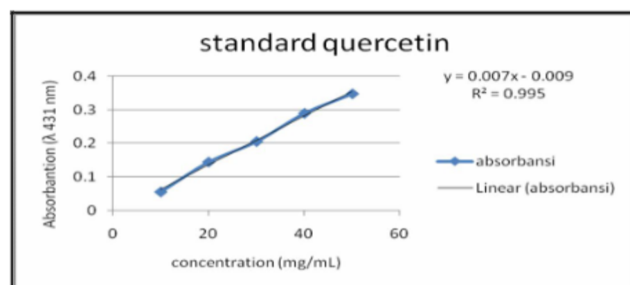
Gambar 2. Standard quercetin curve
