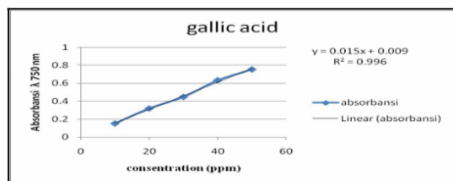
Figure 1. gallic acid curve
