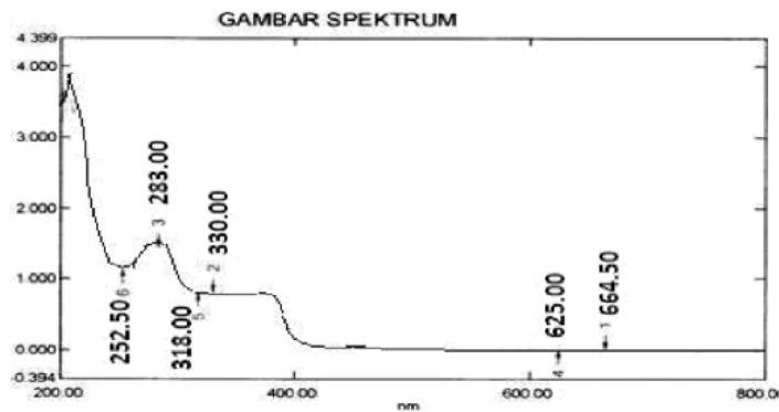
Fig. 3: IR Spectrum of bioactive compound of kopasanda leaf
