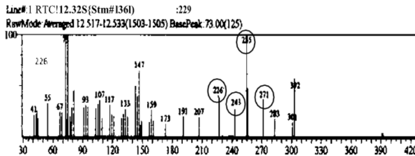
Fig. 5: Analysis of bioactive compounds of kopasanda leaf
