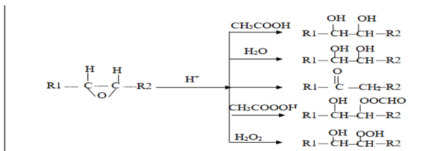
Figure 3. Reaction of Oxirane Ring Degradation by Acids [5].
