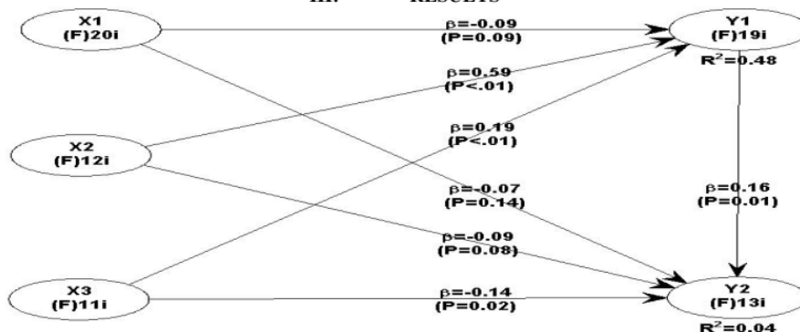
Figure 1. Results Analyze (Inner Model)
