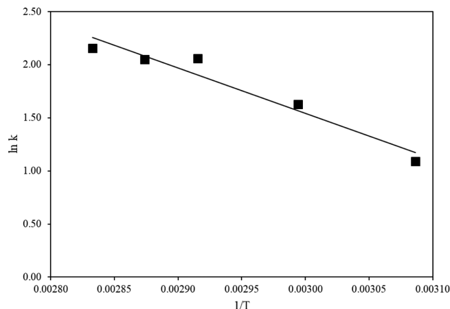
Fig. 6. The relation between \ln k and 1/T (reaction time of 3 min; CaO catalyst of 2.5% (w/w)).
