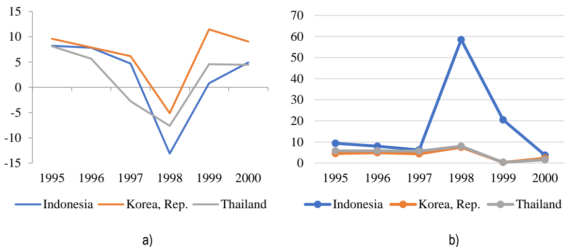
Figure 3. Dynamics of: a) GDP growth; b) annual inflation in selected East Asian countries
