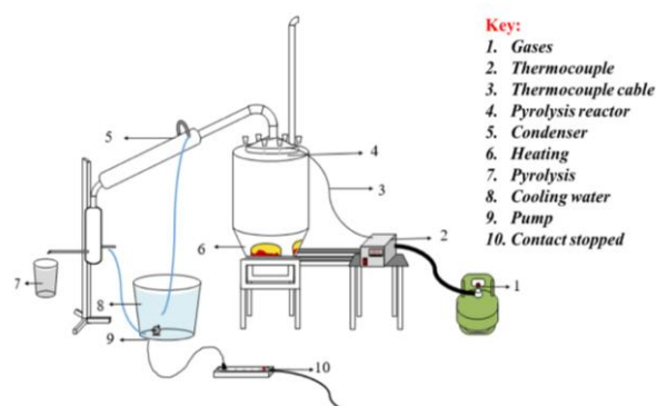
Fig. 2. The schematic illustration of the pyrolysis reactor.
