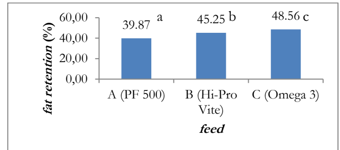
Figure 2. Fat Retention.
