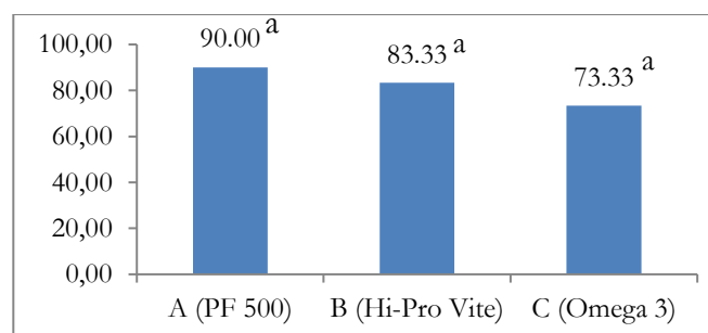
Figure 9. Survival Rate.
