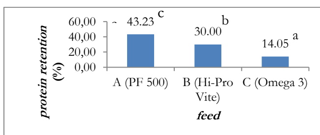
Figure 1. Protein Retention.
